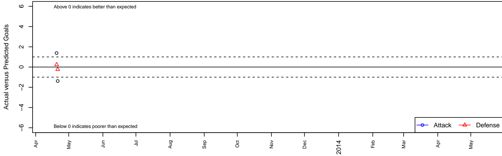
NEU Napoli B00 Dots are actual minus expected GF (blue circles) and GA (red triangles). Blue line is smoothed change in attack strength. Red is smoothed change in defense strength.
